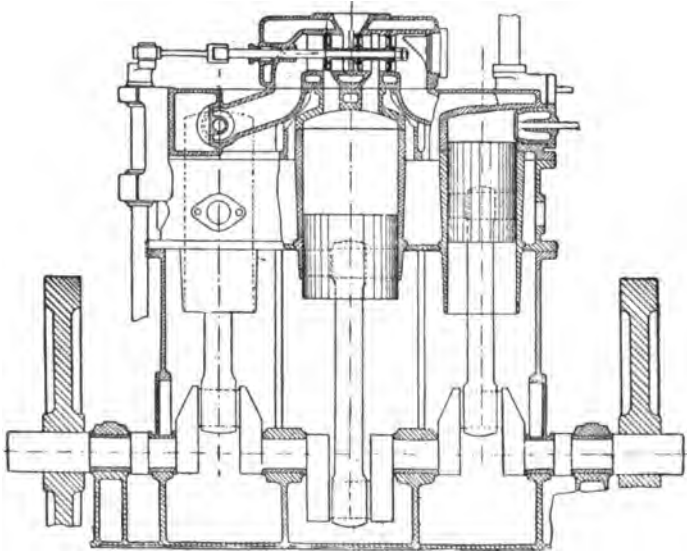
FIG. 306.—Crossley Three-Cylinder Compound Gas Engine. The two end cylinders are high pressure; the central one, low pressure. The exhaust from the two high-pressure cylinders is admitted, alternately, to the low-pressure cylinder by the piston valve, operated by the crank and rotating shaft shown at the left. The exhaust from the low-pressure cylinder passes upward through the port at its top.
